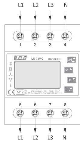
3×230 V+N 3-phase 4-wire installation
