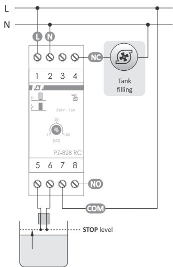
Tank filling
