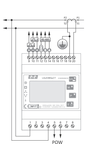
230 V AC 1-phase 2-wire installation
