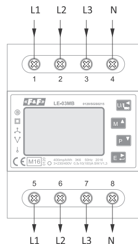
3×400 V 3-phase 3-wire installation (without neutral wire)
