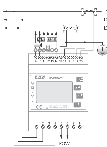
3×400 V 3-phase 3-wire inst. (without neutral wire)
