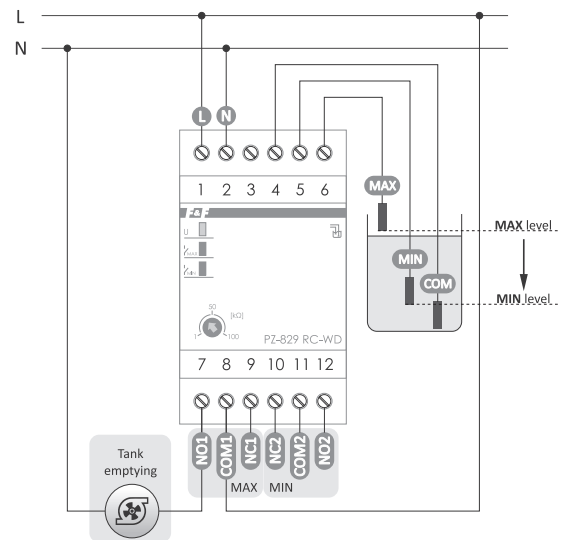
Tank emptying
