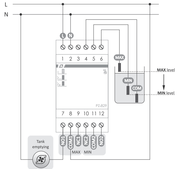
Tank emptying
