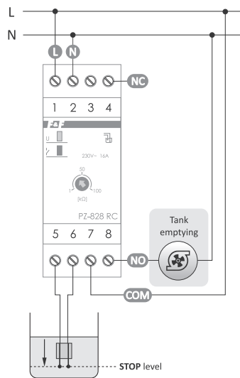
Tank emptying
