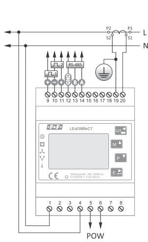
230 V AC 1-phase 2-wire installation
