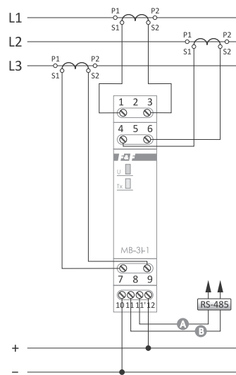
MB-3I-1 5A/MB-3I-1 15A half indirect measurement
